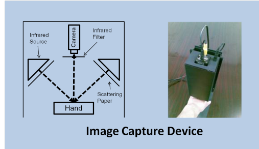
Fig. 1. The setup of the NIR imaging system.
