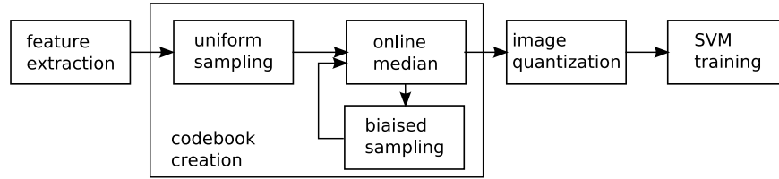
Fig. 11. INRIA-Juric : Outline of the learning steps. See text for details.
