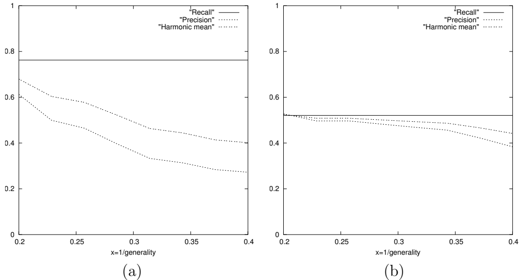
Figure 7: Results on the images shown in figure ??, with varying generality: (a) detection algorithm 1 [?] (b) detection algorithm 2 [?].
