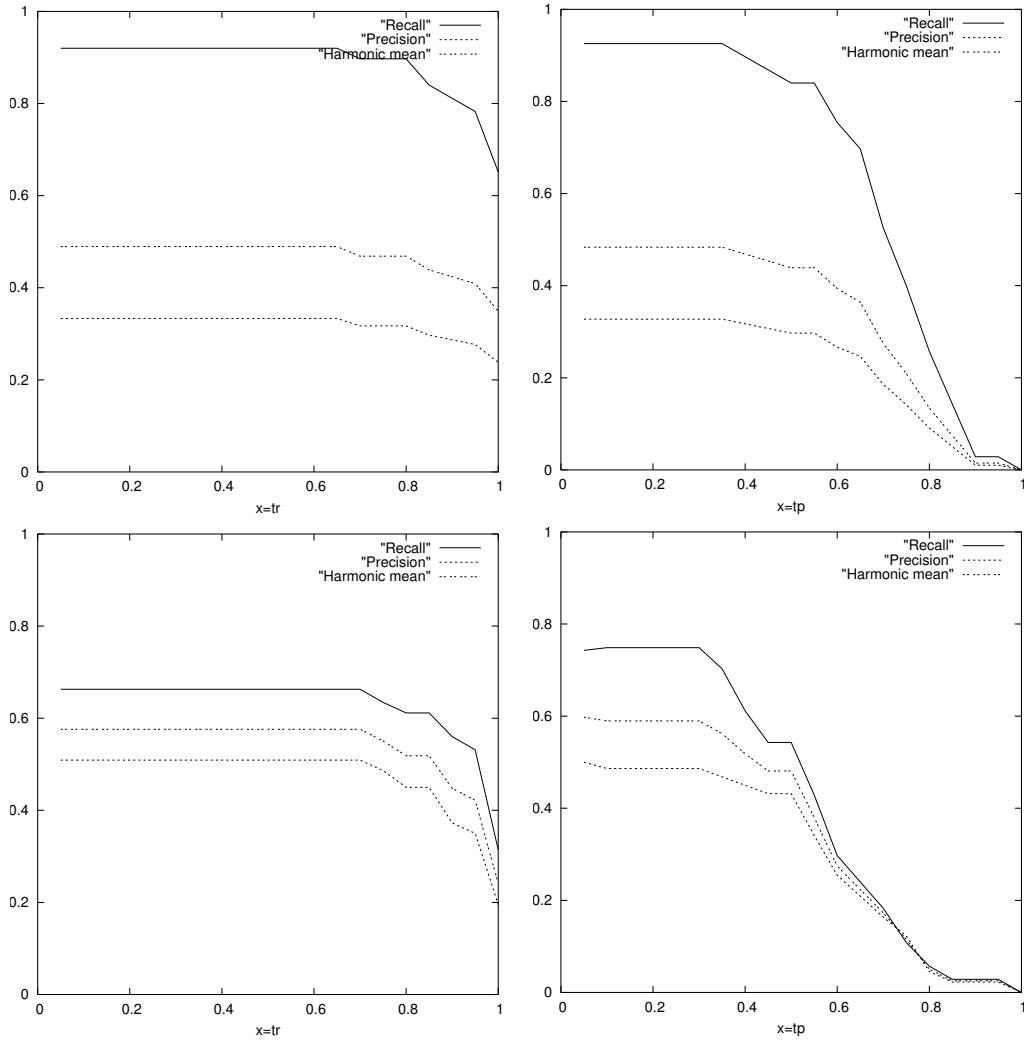
Figure 5: Results on the images shown in figure ?? . Top: detection algorithm 1 [?], bottom: detection algorithm 2 [?]; Left: varying constraint t_r (area recall) while t_p is constant and equal to 0.4, right: varying constraint t_p (area precision) while t_r is constant and equal to 0.8;
