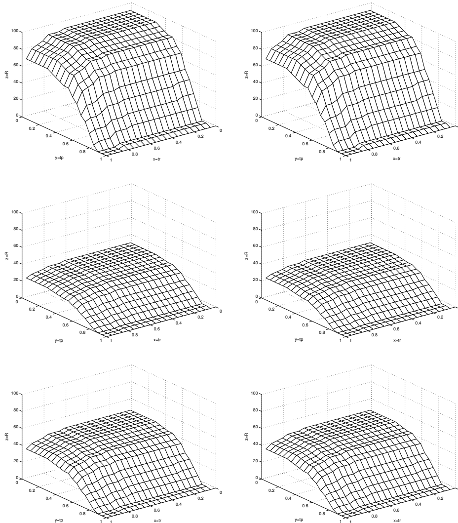
Figure 6: Results on the images shown in figure ???. From top to bottom: recall, precision, harmonic mean. Left: detection algorithm 1 [?], right: detection algorithm 2 [?];
