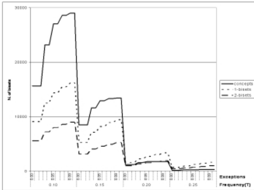
Fig. 3. Characterizing bi-sets for bi-cluster1 in plasmodium w.r.t. different values of minimal size and maximal exception ratio.
