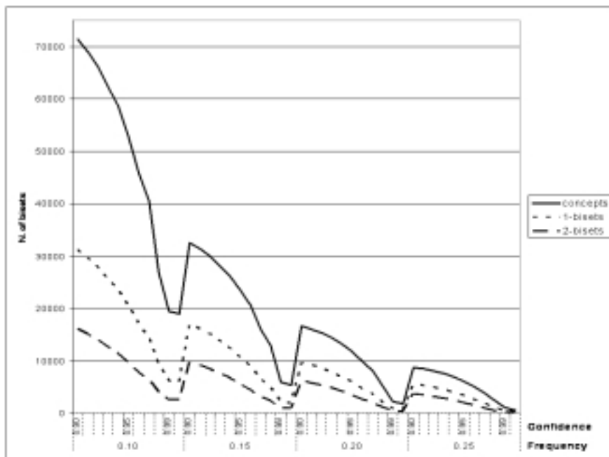
Fig. 4. Characterizing patterns for the bi-cluster2 in meningitis w.r.t. different values of minimal frequency and confidence.
