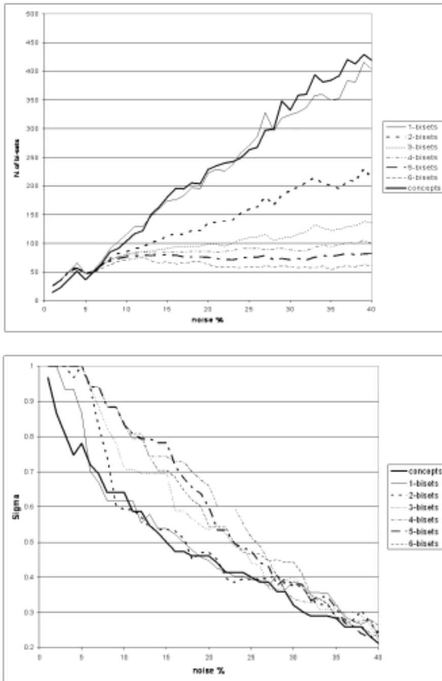
Fig. 1. Size of different collections of bi-sets (top) and related values of \sigma (bottom) depending on noise level.
