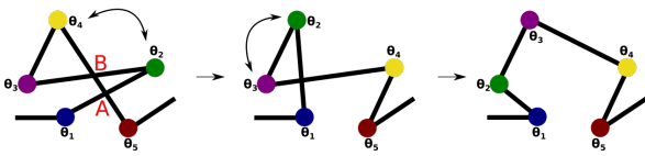
Figure 6: Possible cut intersections are recursively resolved by cone swapping. Here, the intersection A between segments [\theta_1, \theta_2] and [\theta_4, \theta_5] is first solved instead of intersection B because it counts the most intersections between its two extremities \theta_1 and \theta_5 .
