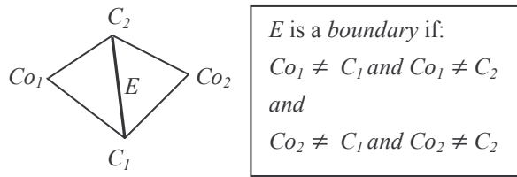
Figure 6. Boundary edge detection for the cracks filling algorithm.
