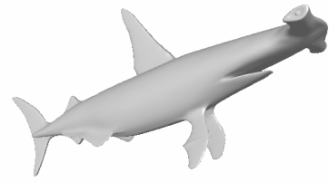
Shark (10234 vertices)
