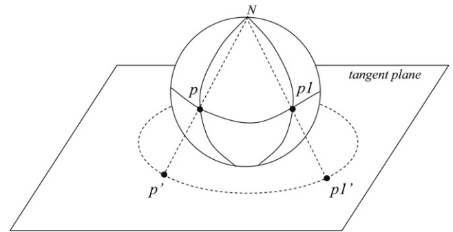
Fig. 10. Stereographic projection used to merge two slope diagrams (revised from [1]).
