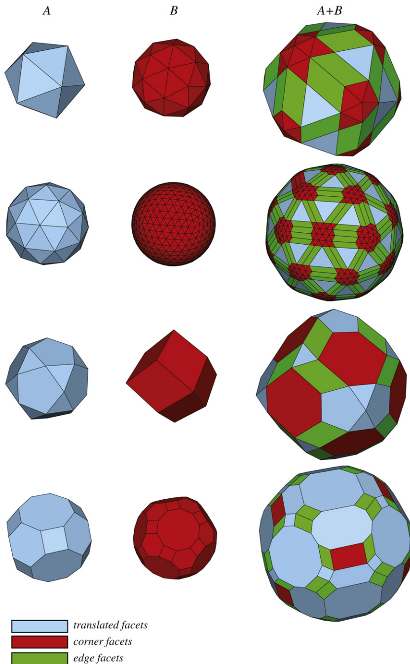
Fig. 13. Minkowski sum examples for convex polyhedra generated by the CVMS algorithm.
