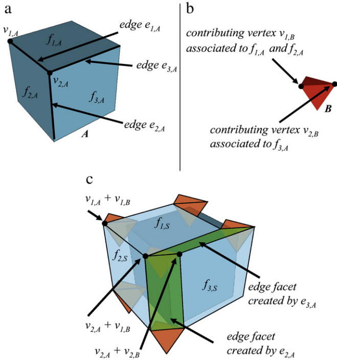
Fig. 7. (a) Some edges e_{1,A} , e_{2,A} , and e_{3,A} of A . (b) Contributing vertices associated to f_{1,A} , f_{2,A} , and f_{3,A} . (c) Edge facets created by e_{2,A} , and e_{3,A} . The edge e_{1,A} will not produce edge facets since incident facets f_{1,A} and f_{2,A} have the same contributing vertex.
