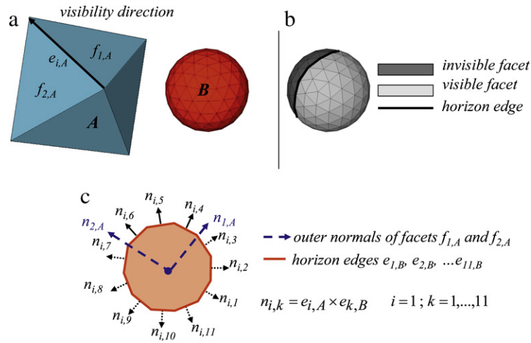
Fig. 8. (a) An edge e_{i,A} as a visibility direction. (b) Visibility computation of all facets of B w.r.t. e_{i,A} and horizon edges determination. (c) Only horizon edges e_{4,B} , e_{5,B} , and e_{6,B} will produce edge facets e_{i,A} \oplus e_{4,B} , e_{i,A} \oplus e_{5,B} , and e_{i,A} \oplus e_{6,B} .
