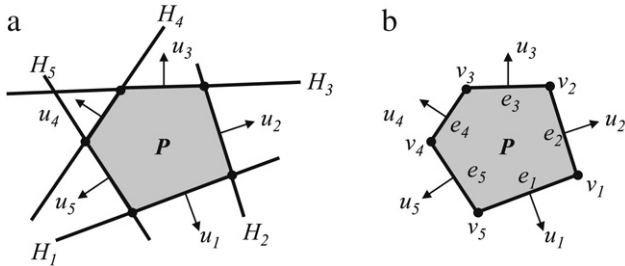
Fig. 2. The intersection of closed half-planes. (a) A finite number of closed half-planes H_1, \dots, H_5 defined by H_1, \dots, H_5 . (b) The boundary of P is partitioned into 1D faces (edges) e_1, \dots, e_5 and 0D faces (vertices) v_1, \dots, v_5 .
