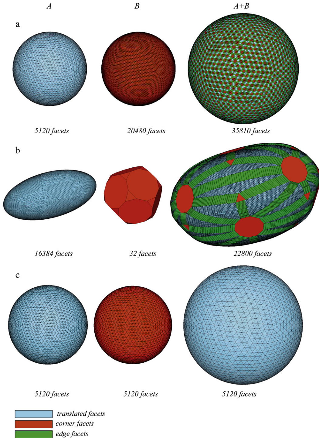
Fig. 14. More results of the CVMS algorithm for: (a) Two spheres having thousands and tens of thousands of facets. (b) An ellipsoid-like polyhedron and a truncated dodecahedron. (c) For an extreme degenerate case (two identical spheres with thousands of facets).
