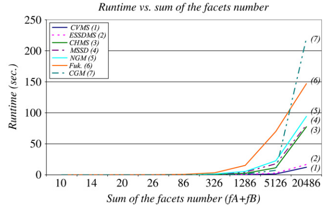
Fig. 12. Evolution of the running time of the algorithms mentioned in Table 1 with respect to the sum of the number of facets of the operands. This figure shows that when increasing the number of facets, the CVMS and the ESSDMS algorithms are largely preferred in comparison to other algorithms.
