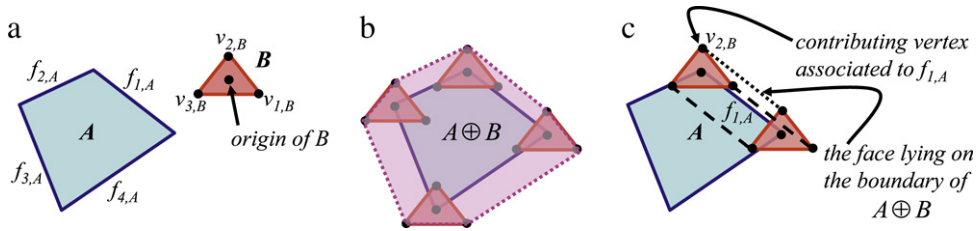
Fig. 3. (a) Two convex polygons A and B . (b) The Minkowski sum A \oplus B depicted as a sweep. (c) The contributing vertex v_{2,B} associated to the face f_{1,A} . The dotted line is the face that lies on the boundary of A \oplus B . The two other faces (dashed lines) are discarded.
