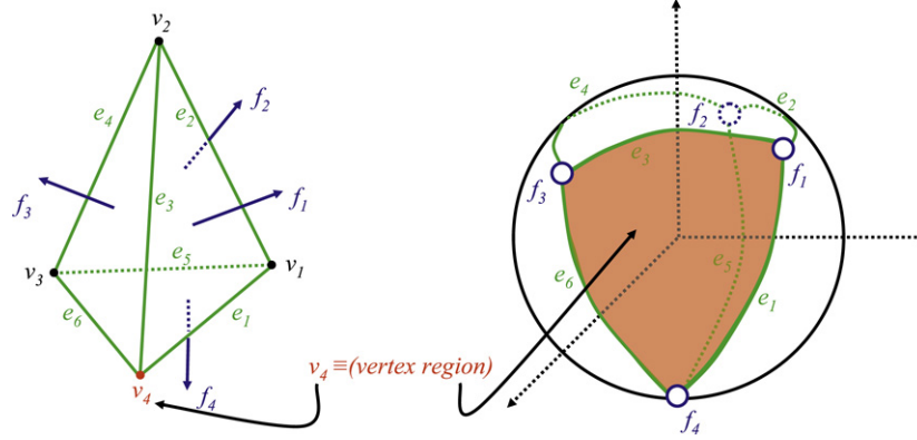
Fig. 9. A convex polyhedron and its slope diagram representation (revised from [1]).
