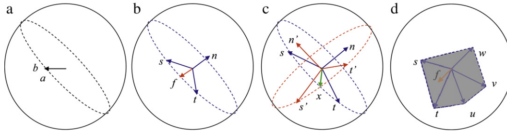
Fig. 11. Intersections in slope diagrams. (a) Intersection of two facet points. (b) Intersection of a facet point and an edge arc. (c) Intersection of two edge arcs. (d) Intersection of a facet point and a vertex region.
