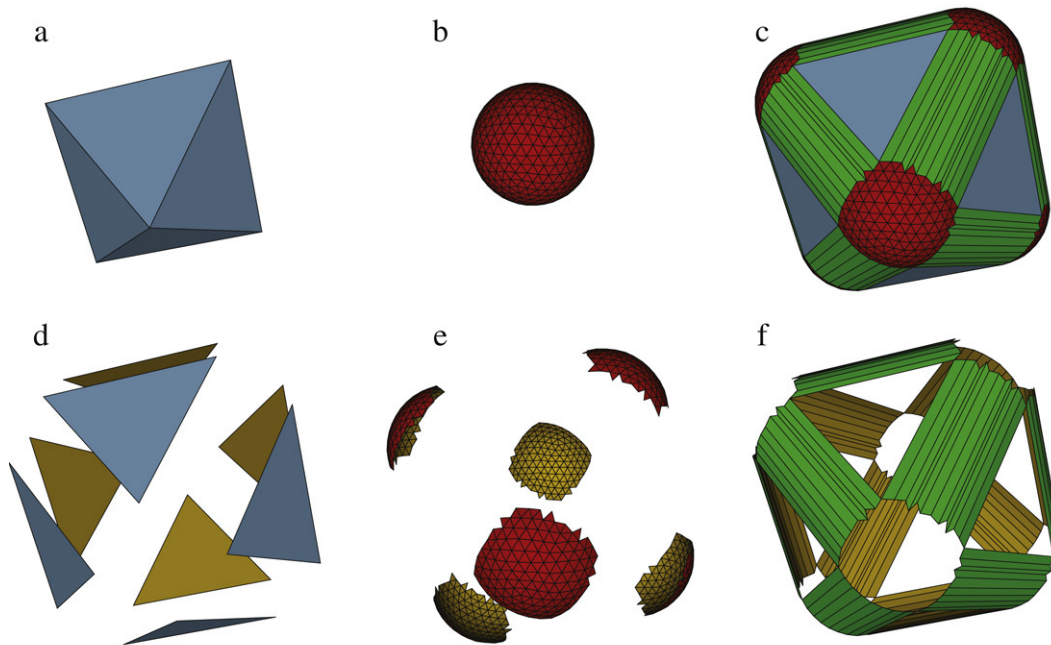
Fig. 6. (a) Polyhedron A. (b) Polyhedron B. (c) Sum polyhedron S. (d) Translated facets. (e) Corner facets. (f) Edge facets.
