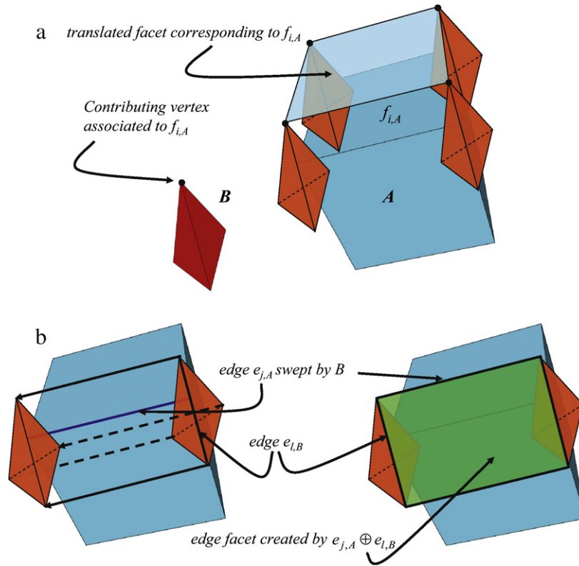
Fig. 5. (a) The creation of a translated facet corresponding to a particular facet f_{i,A} and its associated contributing vertex (the corner facets are determined in the same manner). (b) Sweeping an edge e_{j,A} by B and creation of an edge facet e_{j,A} \oplus e_{i,B} .
