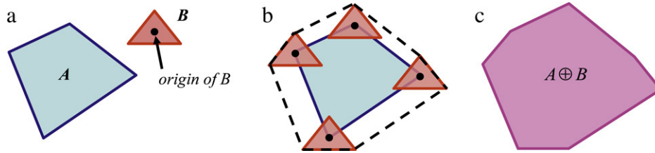
Fig. 1. Minkowski sum as a sweep of two sets. (a) Two polygons A and B . (b) B is positioned on each point of A . (c) The Minkowski sum A \oplus B is the union of the resulting translations of B on all points of A .
