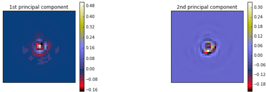
Figure 10. PCA-learned components.
