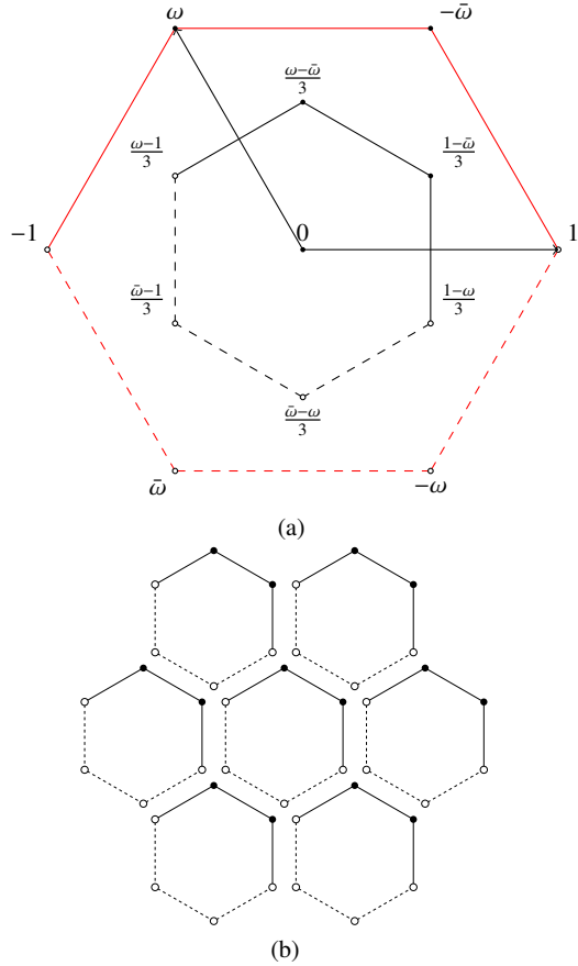
Fig. 4 In (a) visualization of hexagonal cells: \mathcal{C}_1(0) (in black) \mathcal{C}_{(2+\omega)}(0) (in red). Dashed lines and white circles—which represents points—are not included in hexagonal cells. (b) illustrates the adjacency of the sides and the vertices of hexagonal cells. The space between the hexagonal cells has been added for a visualization purpose.
