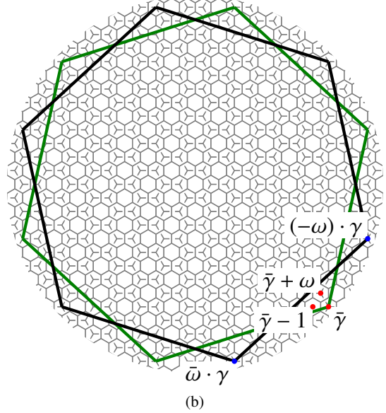
Fig. 8 Visualization of C_{\gamma(2+\omega)}(0) and C_{\bar{\gamma}(2+\omega)}(0) for: s = 3, t = 5 (a); s = 4, t = 9 (b), depicted in black and green, respectively. The usual hexagonal grid is depicted in gray, whereas its mapping by 2 + \omega is depicted in gray and represented by dashed line segments
