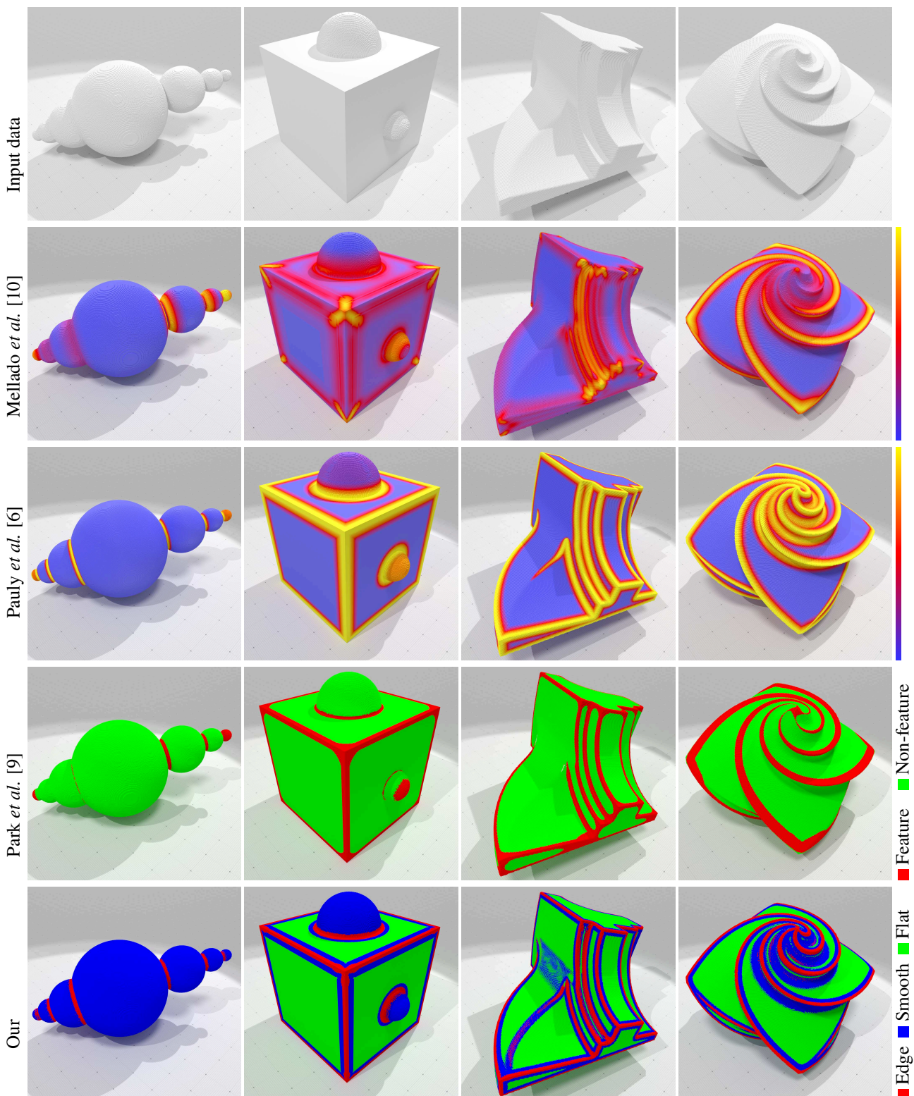
Figure 9: Evaluation of feature detectors on perfectly digitized shapes. SpheresUnion: 400 \times 200 \times 200 voxels, CubeSphere: 200^3 voxels, Fandisk: 512^3 voxels, OctaFlower: 512^3 voxels. Parameters used for [10]: r_{min} = 5 , r_{max} = 25 . Parameters used for [6]: r_{min} = 5 , r_{max} = 25 , \tau_{max} = 0.01 . Parameters used for [9]: r_{min} = 5 , r_{max} = 25 , \omega_{min} = 1.4 , \omega_{max} = 1.4 , \tau = 1.2 . Parameters used for our algorithm: r_{min} = 5 , r_{max} = 25 .
