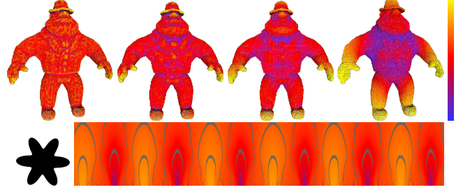
Figure 2: Top : Mean curvature using Eq. 6 for different ball radii: 4, 7, 14 and 30. Bottom : 2D flower and curvature values on its boundary using Eq. 5 (x-axis) for a range of decreasing ball radii (y-axis, from top to bottom). Curvature values are mapped from blue (lower) to yellow (higher), discrete gray lines illustrate curvature isovalues.
