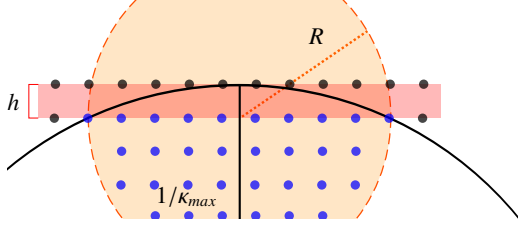
Figure 5: Digitization effect and notations for Property 1.
