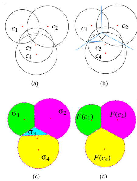
Fig. 4. Digital stable manifold construction: (a) input set of medial balls with centers c_1, c_2, c_3 and c_4 , (b) and (c) depict the corresponding power diagram and their associated cells \sigma_1, \sigma_2, \sigma_3 and \sigma_4 , c_3 \notin \sigma_3 , being regular, we have l(c_1) = 1, l(c_2) = 2, l(c_3) = 4 , and l(c_4) = 4 . (d) illustrates the associated stable manifolds.
