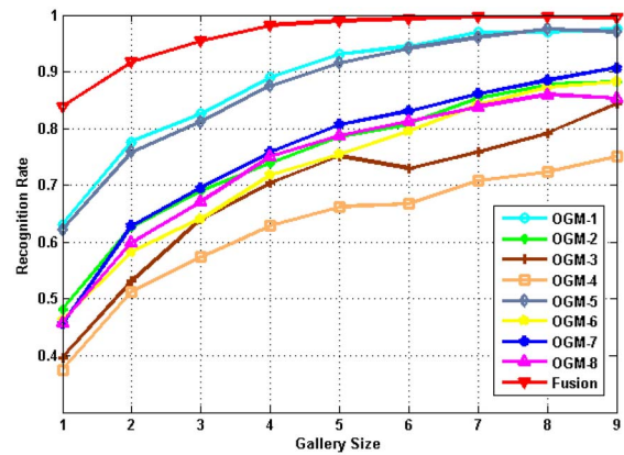
Fig. 12. Accuracy curves based on individual OGMs and their combination with respect to the gallery size of each subject on NCUT Part A.
