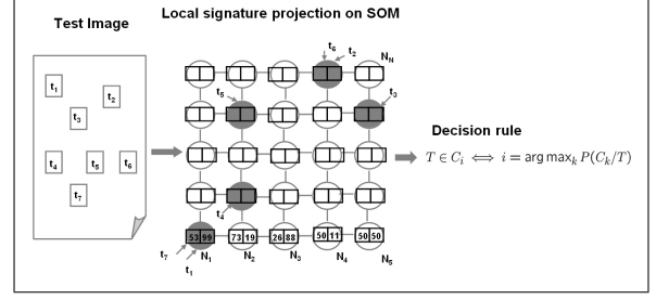
Figure 4. Decision rule.
