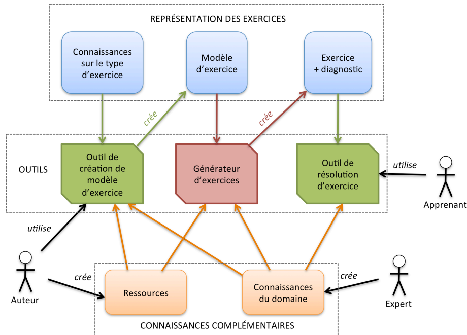
Figure 2. Architecture de notre approche
