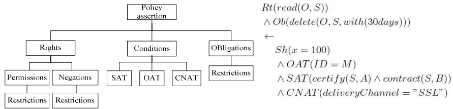
Fig. 3. The context-aware security policy model and a sample policy in concise syntax.
