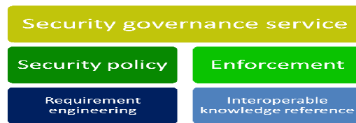
Fig. 1. Framework overview.
