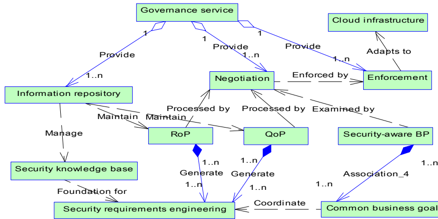
Fig. 2. Framework model.
