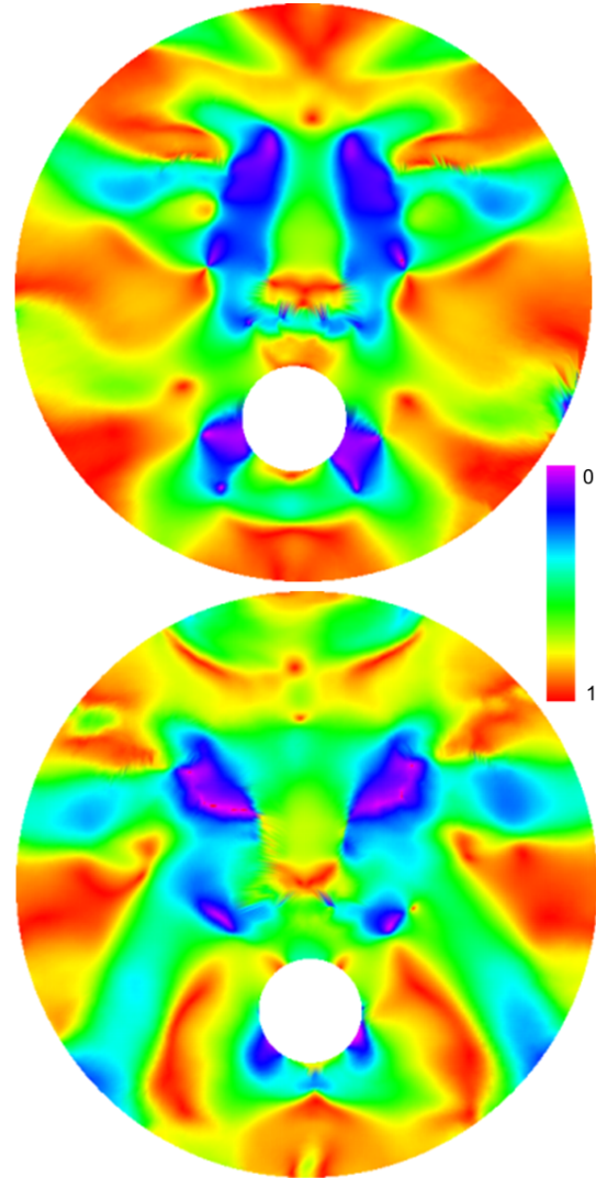
Figure 8. Conformal maps (Figure 2) transformed by Möbius transformation with center point in the nose tip.
