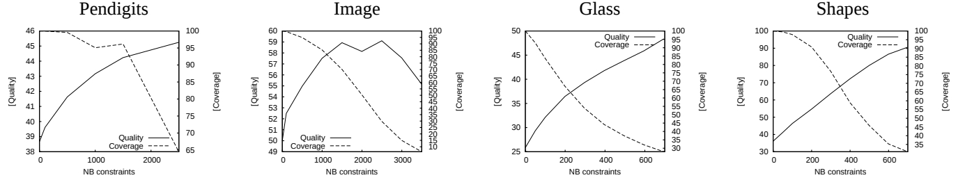
Figure 9: SC-CLIQUE: quality (%) and coverage (%) as the number of instance-level constraints increases.
