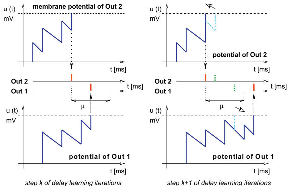
Fig. 3. An example illustrating the effect of one iteration of the delay learning algorithm on the firing times of the two readout neurons.
