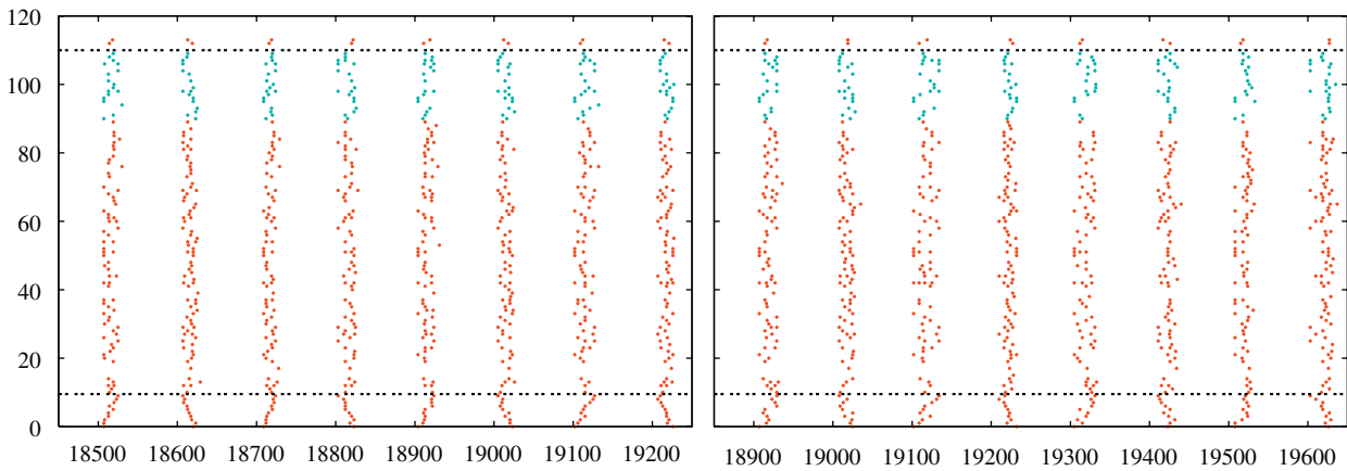
Fig. 6. Spike raster plots, for two series of noisy patterns: \eta = 4 (top) and 8 (bottom).
