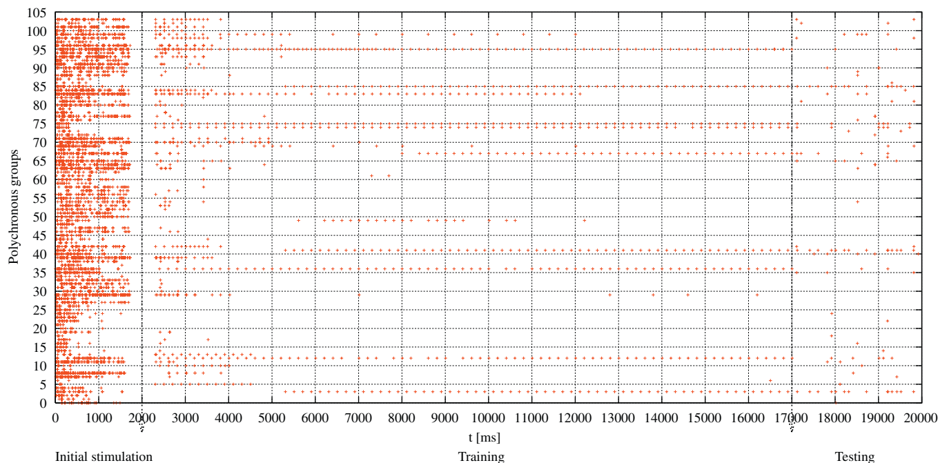
Fig. 12. Evolution of polychronous groups activation during the initialization, learning and generalization phases of experiments reported in Section 4.1, with alternate class input presentations. Note that, in this figure, the y -axis represents the PG indices and no longer the neuron indices, as was the case on spike raster plots.
