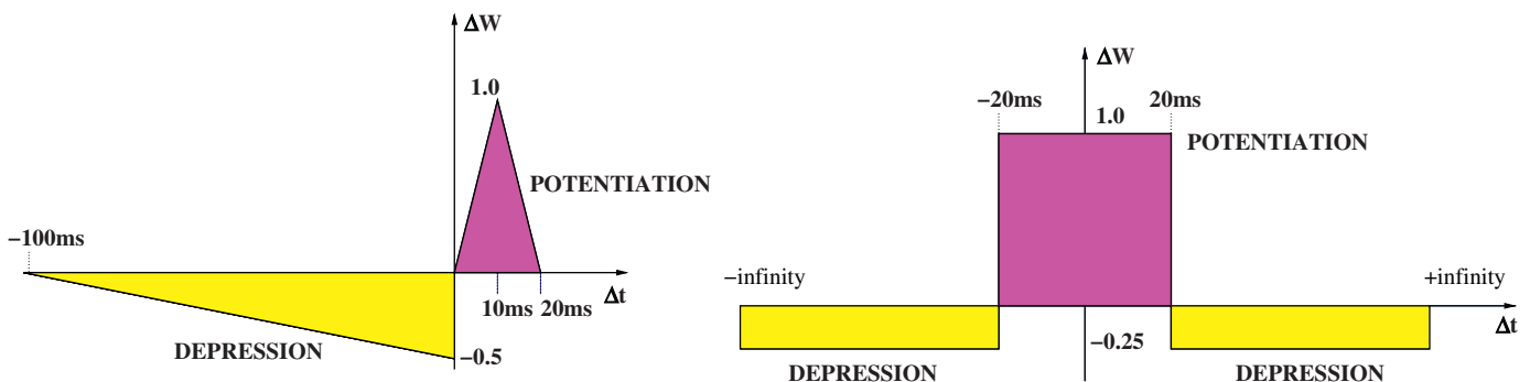
Fig. 2. Asymmetrical STDP temporal window for excitatory (left) and symmetrical STDP temporal window for inhibitory (right) synapse adaptation (from [29]).
