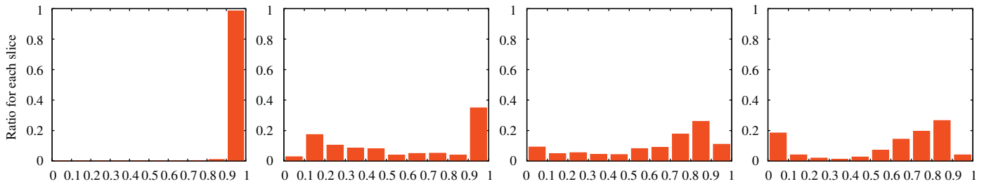
Fig. 8. Distribution of |w_{ij}| for inhibitory weights at time 300, 2000, 4000, 10000 ms.
