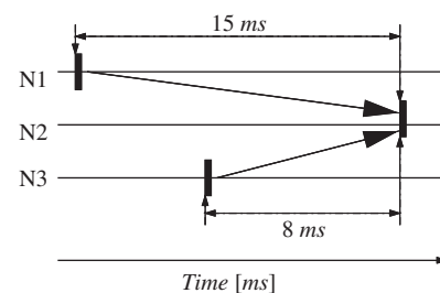
Fig. 10. Example of two triggering neurons giving rise to a third one firing.
