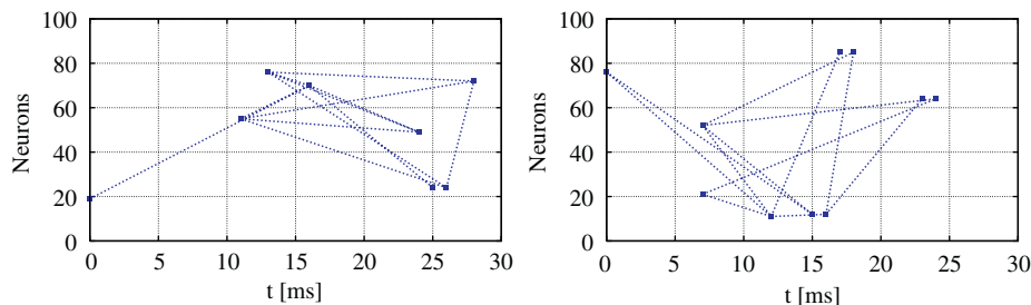
Fig. 11. Examples of polychronous groups: PG_50 and PG_51. Starting from three initial triggering neurons, further neurons of the group can be activated, in chain, with respect to the spike-timing patterns represented on the diagrams.
