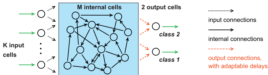
Fig. 1. Architecture of the spiking neuron network. The reservoir is the internal network (the colored square) and green (light gray) links represent the interface with environment. The network is presented for C = 2 classes.
