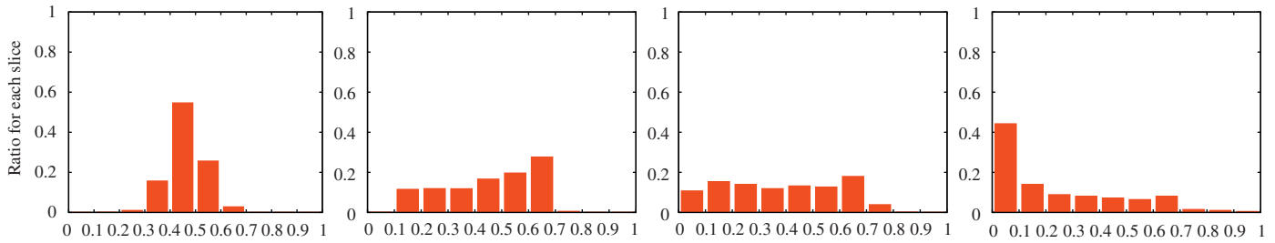
Fig. 7. Excitatory weights distribution at time 300, 2000, 4000, 10000 ms.
