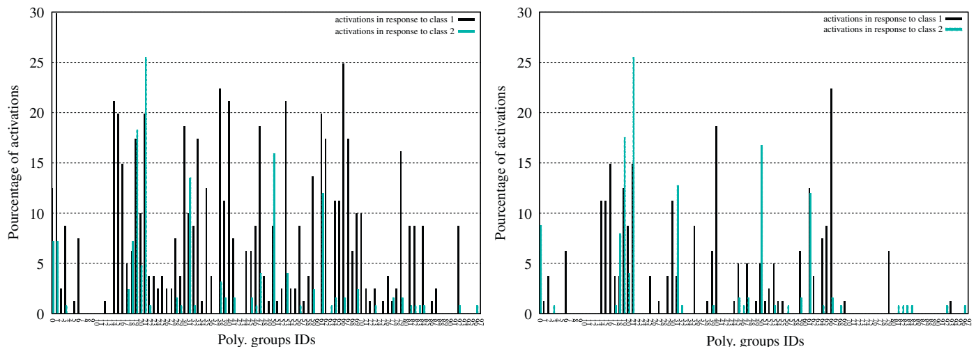
Fig. 15. Activation ratio of PGs in a 100 neurons reservoir, for two-class discrimination of USPS digits 1 versus 9, during the 1st (left) and the 5th (right) epochs.
