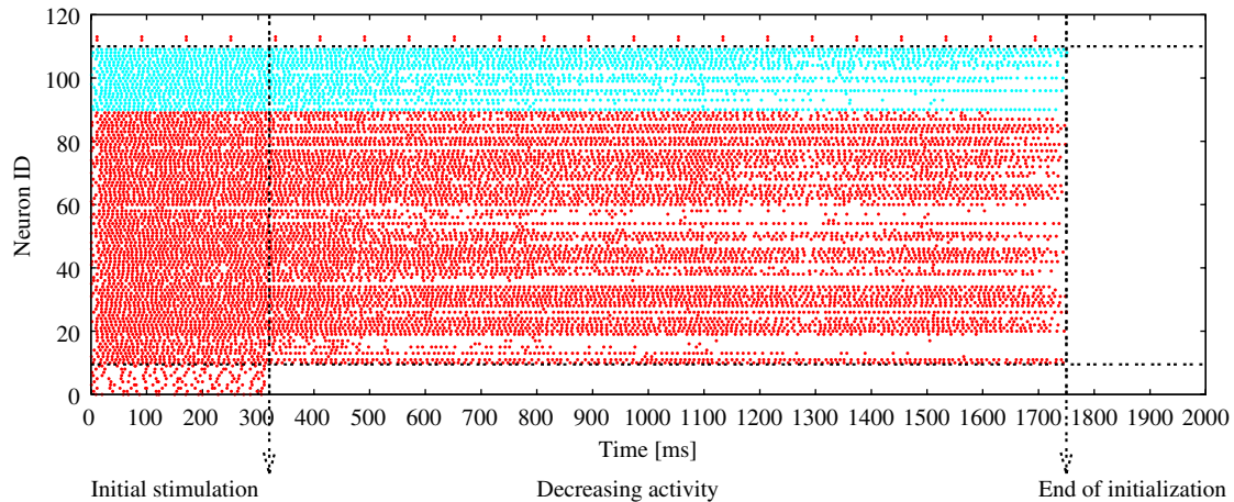
Fig. 4. Spike raster plot, for initial random stimulation, from time 0 to 2000 ms.
