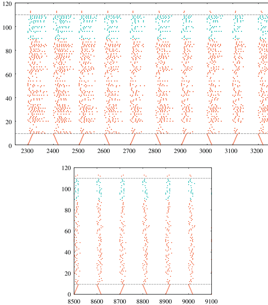
Fig. 5. Spike raster plots, for two time slices of a learning run, one just after T_{L1} (top) and the other a long time after activity has stabilized, until T_{L2} (bottom).
