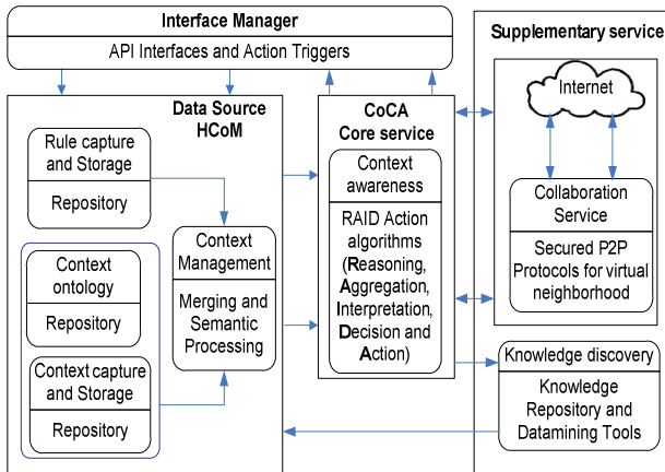
Fig. 4 Architecture for the CoCA platform
