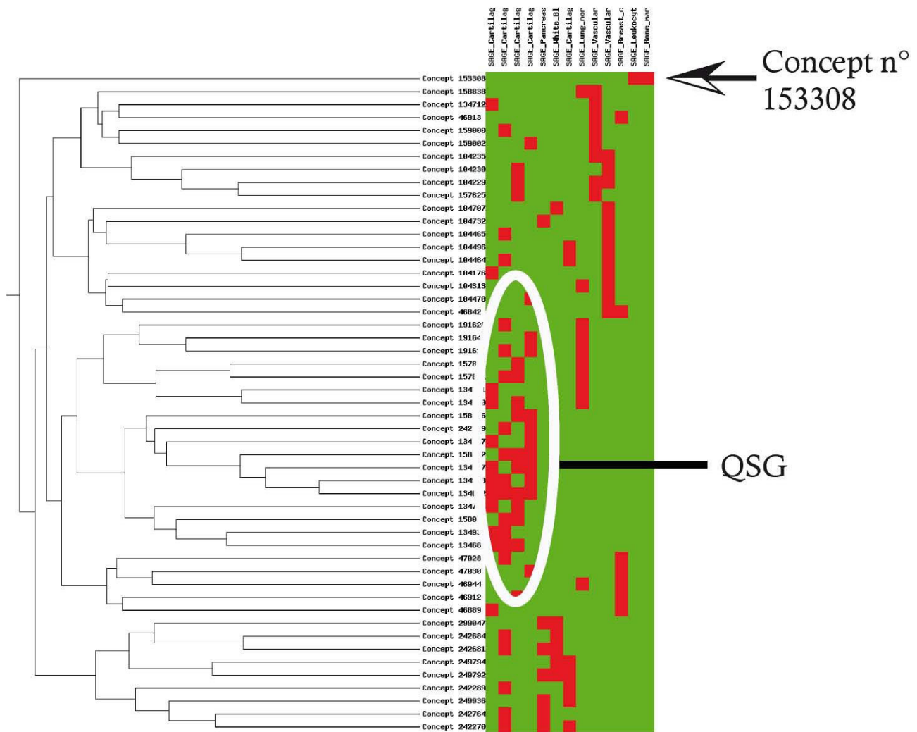
Figure 4 Hierarchical clustering analysis of the 51 formal concepts. The concepts shown on the left are represented according to the libraries they contain (shown on top). A red square indicates a library within a concept, a green square a library not within the corresponding concept. From the hierarchical clustering shown on the left, one concept appears to be very different from the rest (n° 153308), and a group of concept appears sufficiently similar to be grouped within a QSG.
