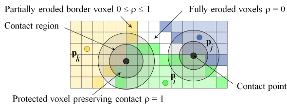
Figure 18: Erosion of the discrete Voronoi volumes
