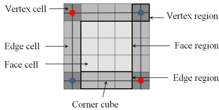
Figure 8: The corner cube grid structure ( n = 5 )
