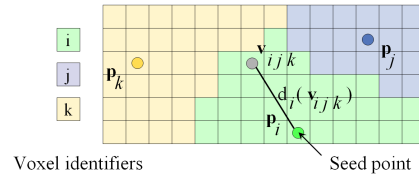
Figure 14: Erosion of the discrete Voronoi volumes
